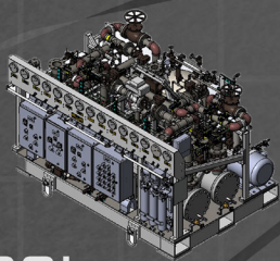
FIRE CONTROL SYSTEM WATER COOLERS
